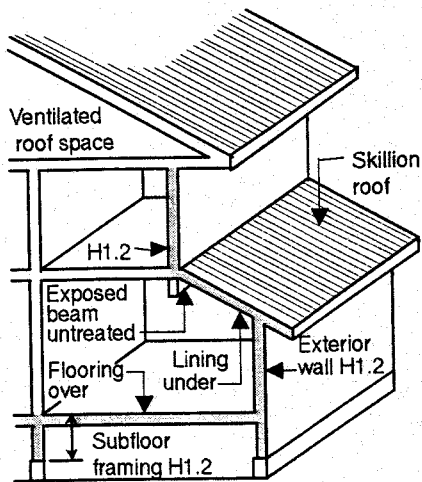
General wall and roof framing
